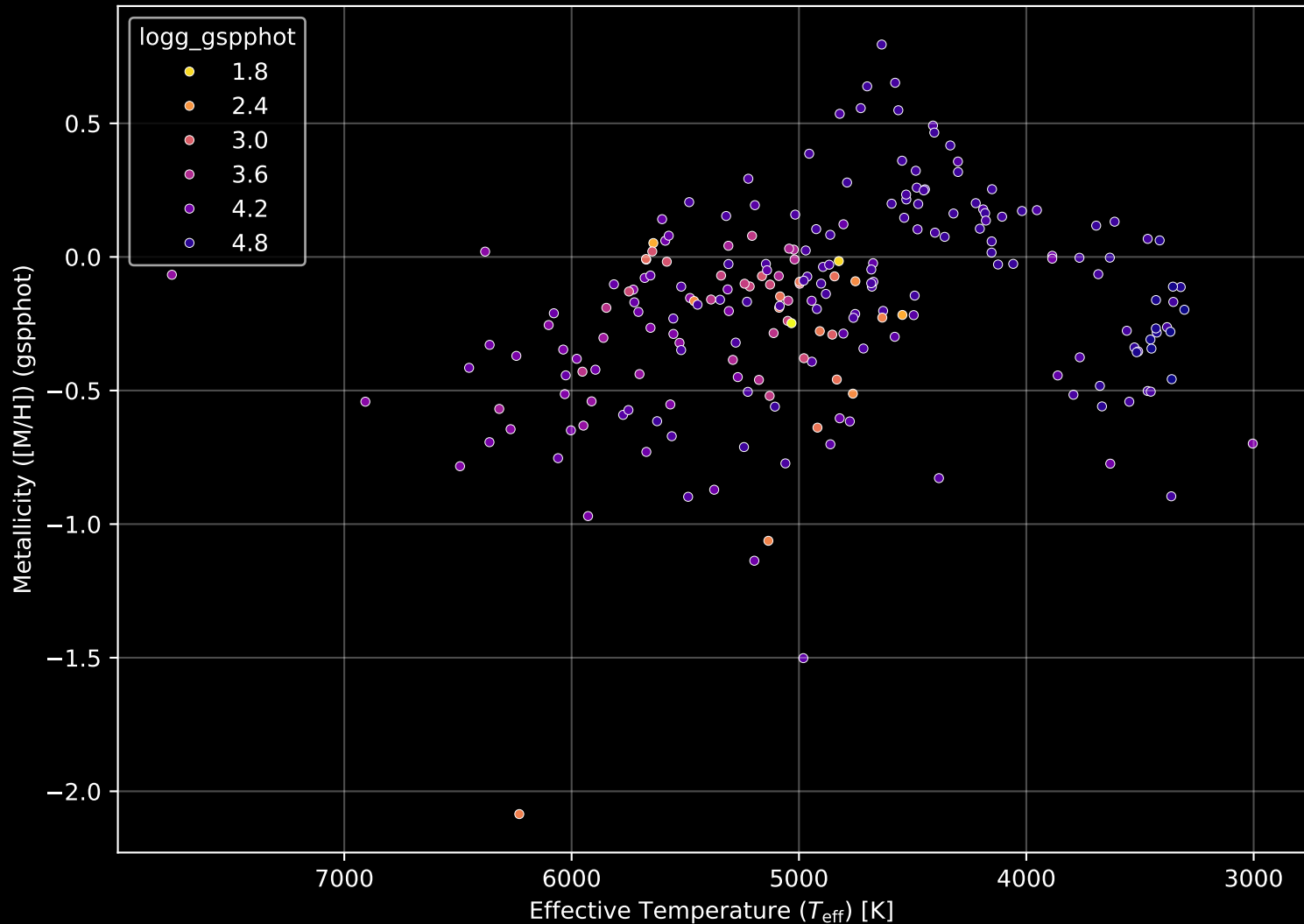
APOGEE DR17 Field: [K2_C14_234+49] Stellar Population Parameters (n= 221)
