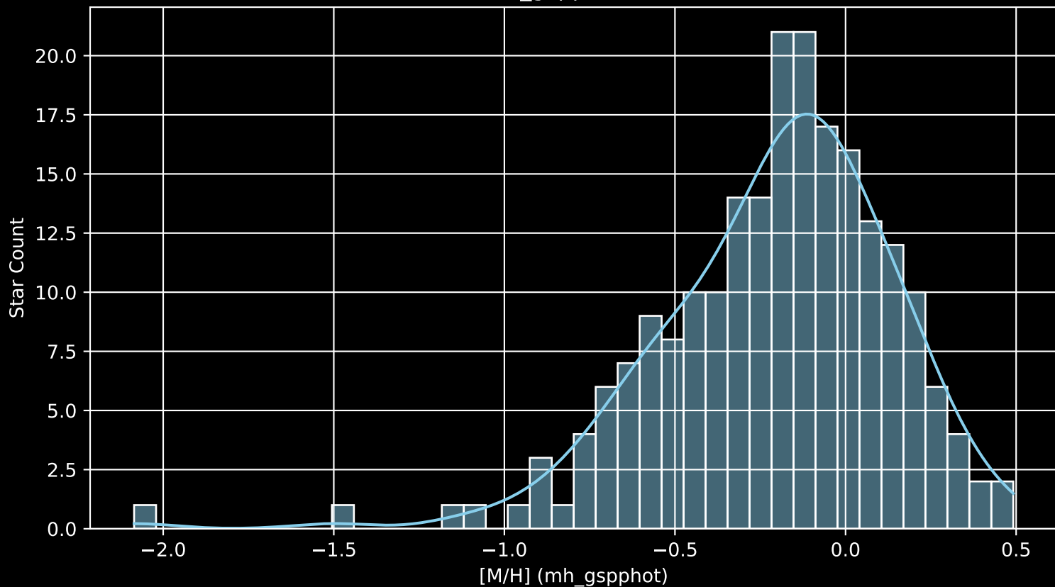
APOGEE DR17 Field: [K2_C14_234+49 [M/H] (mh_gspphot) (n= 215)
