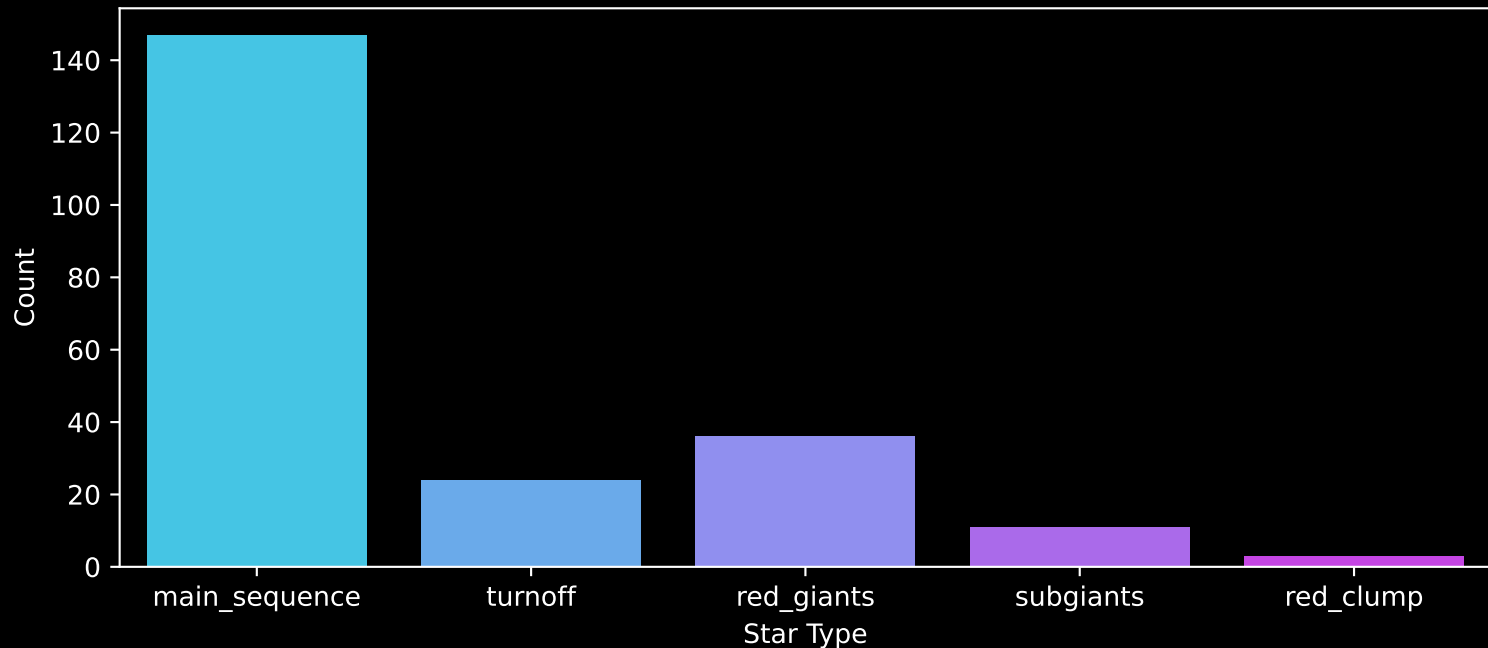
APOGEE DR17 Field: [K2_C14_234+49] Count plot of Star Type
