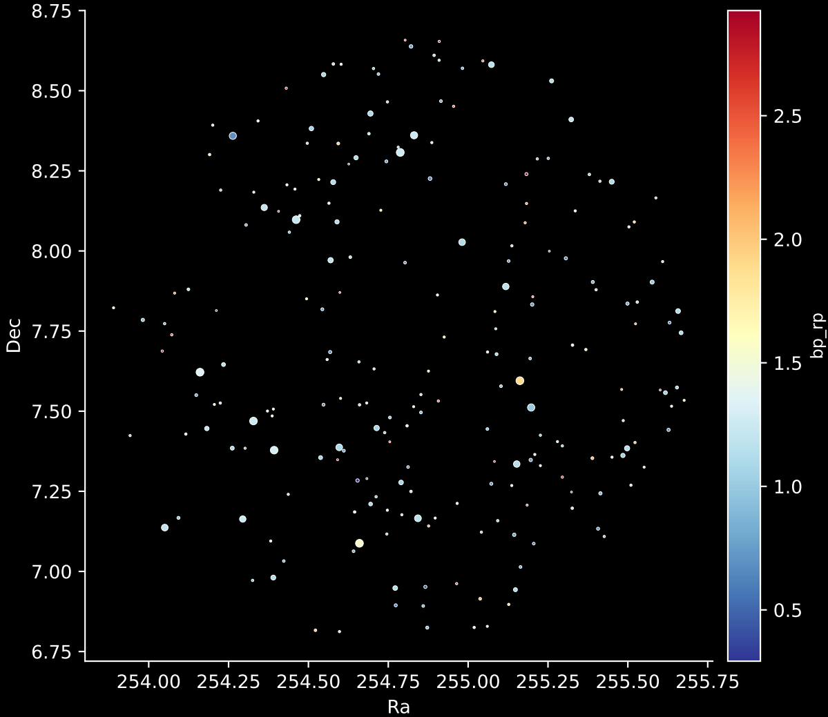
APOGEE DR17 Field: [K2_C14_234+49] Stars: 221
