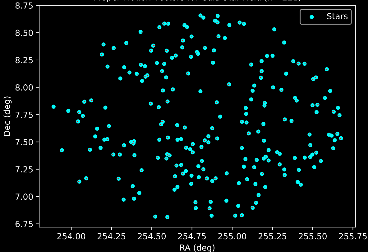
APOGEE DR17 Field: [K2_C14_234+49] Proper Motion Vectors for Gaia Star Field (n= 221)
