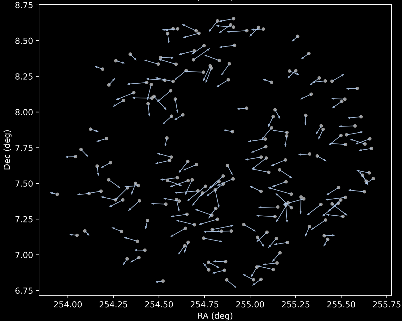
APOGEE DR17 Cluster 1 Proper Motion Vectors (n=182)
