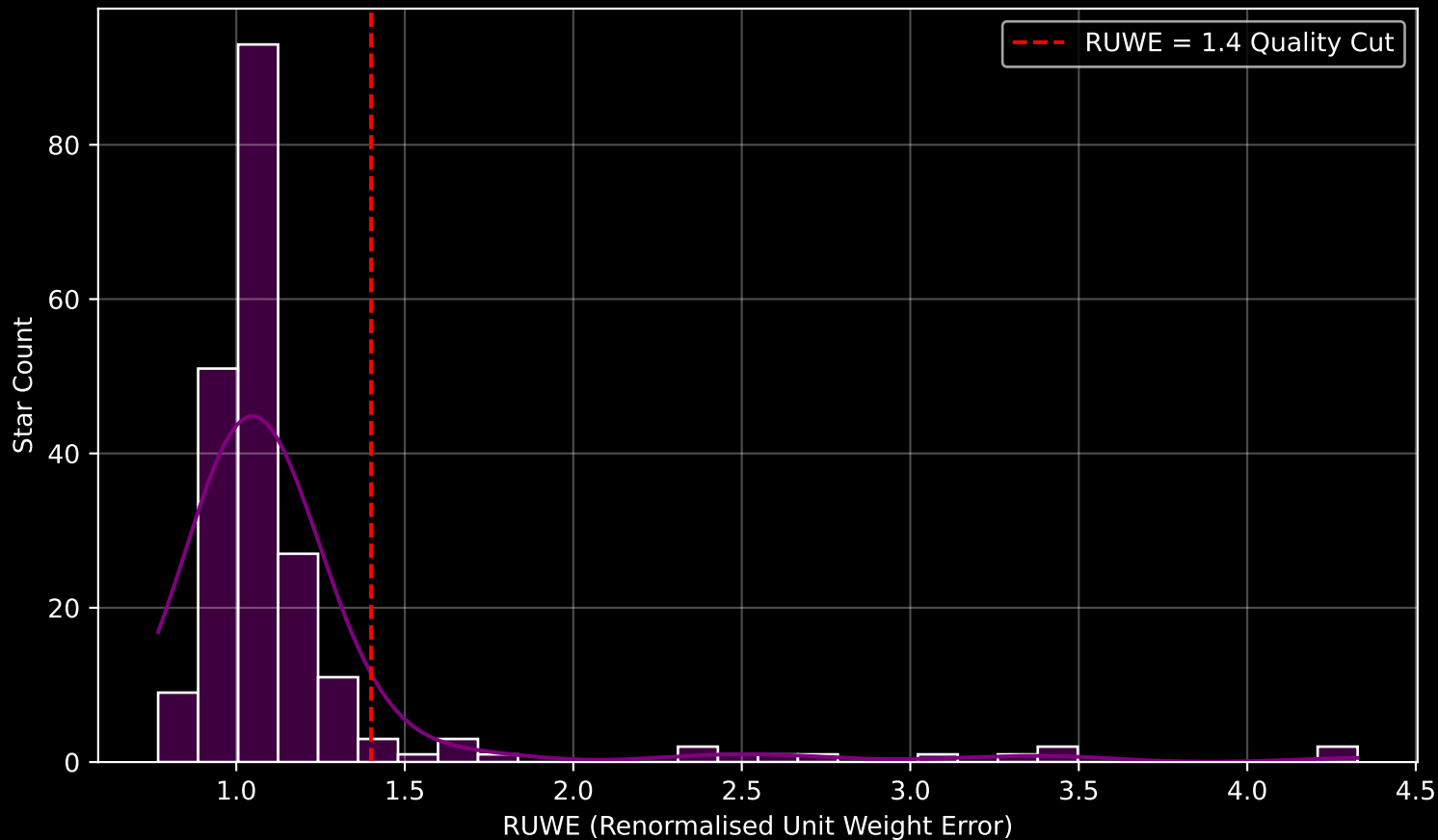
GAPOGEE DR17 Field [K2_C14_234+49] RUWE Distribution (n= 210)
